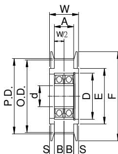
Two Bearings
