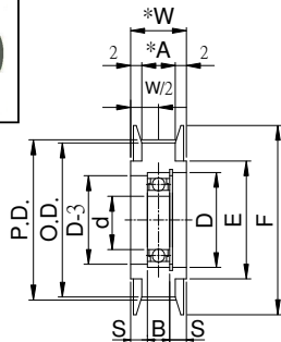
One Bearing
